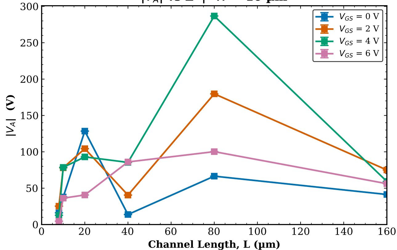
TFT3 Transistor 2 |V_A| vs L | W = 10\text{ }\mu\text{m}
